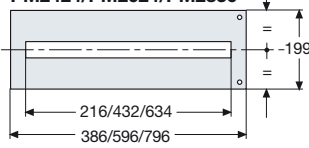
Version for Tmax with mod. diff. PM2312/PM2315
