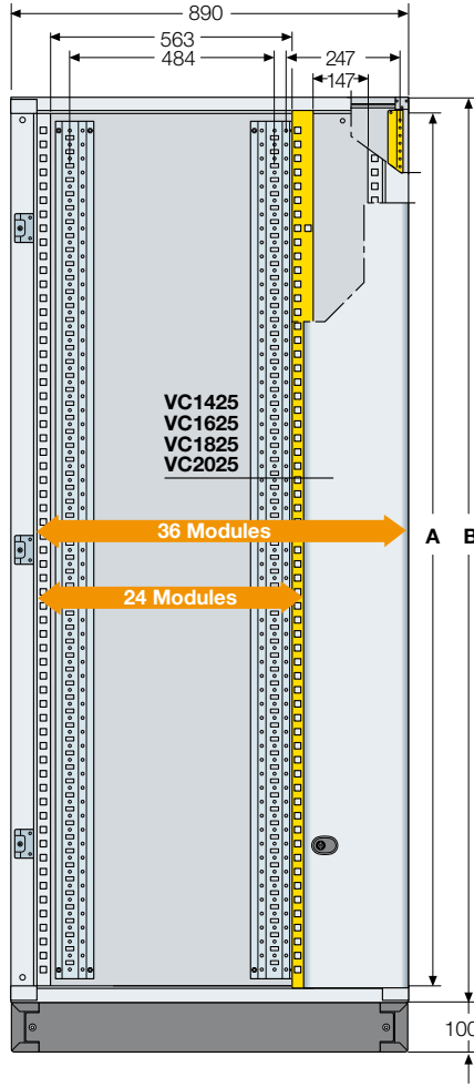
Front of structure with internal cable container
