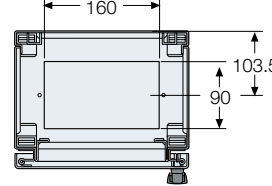
Base of cable container
