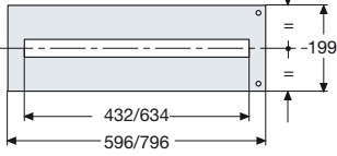
Version for Tmax with mod. diff. PM2312/PM2315
