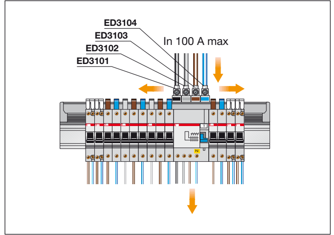
Busbar power supply by means of power supply terminals placed laterally
