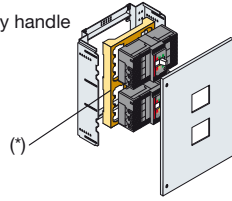
Tmax interlocked or interlocked motor operated
