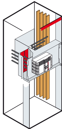
Form 4 (separation of the busbars from the functional units + separation of the functional units from each other + separation of the terminals from each other)
