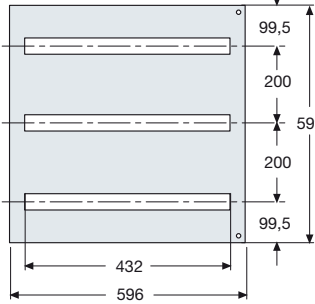
Width 600/800mm PS4720/PS4728/PS4960/PS4968
