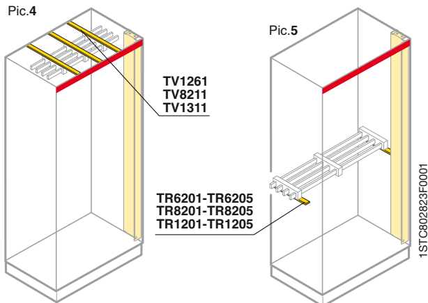
Pic. 5 Busbars horizontally at any height in the structure
