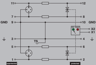
Complete module, direct earthing, with remote alert
