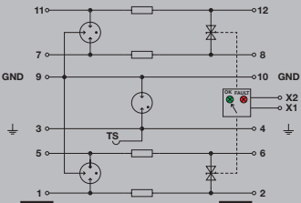
Complete module, indirect earthing, with remote alert
