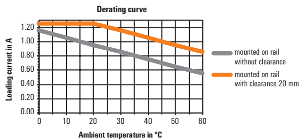
Derating curve MCZ OVP I_{\max} = 1,25\text{ A}
