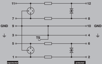
Complete module, direct earthing
