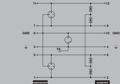
Complete module, indirect earthing
