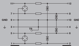
Complete module, direct earthing
