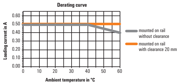
Derating curve MCZ OVP I_{\max} = 0,5\text{ A}
