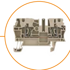
Z系列弹片接线技术 Z series tension clamp connection technology
